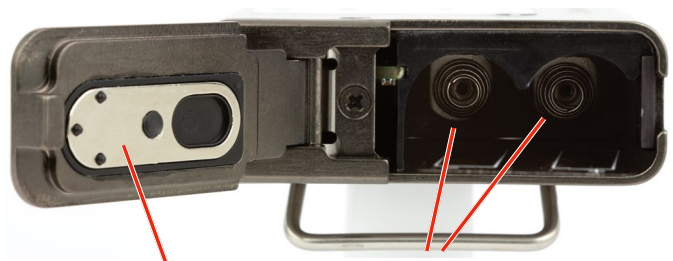
Series connection plate
